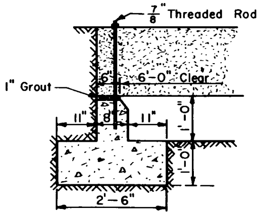
SECTION G-G TYPICAL LONGITUDINAL SUPPORT
